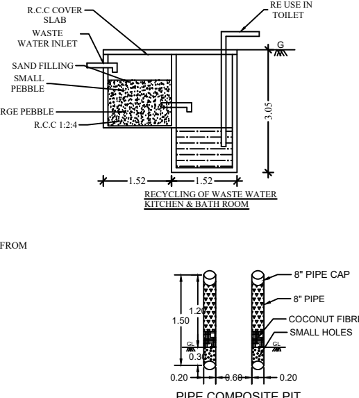
PIPE COMPOSITE PIT
