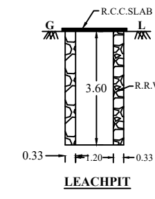
LEACHPIT
