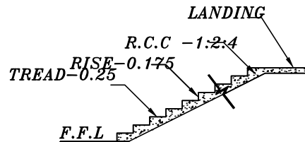
STAIRCASE DETAIL
