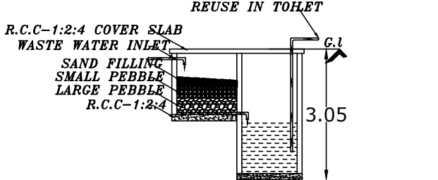
RECYCLING OF WASTE WATER KITCHEN & BATH ROOM
