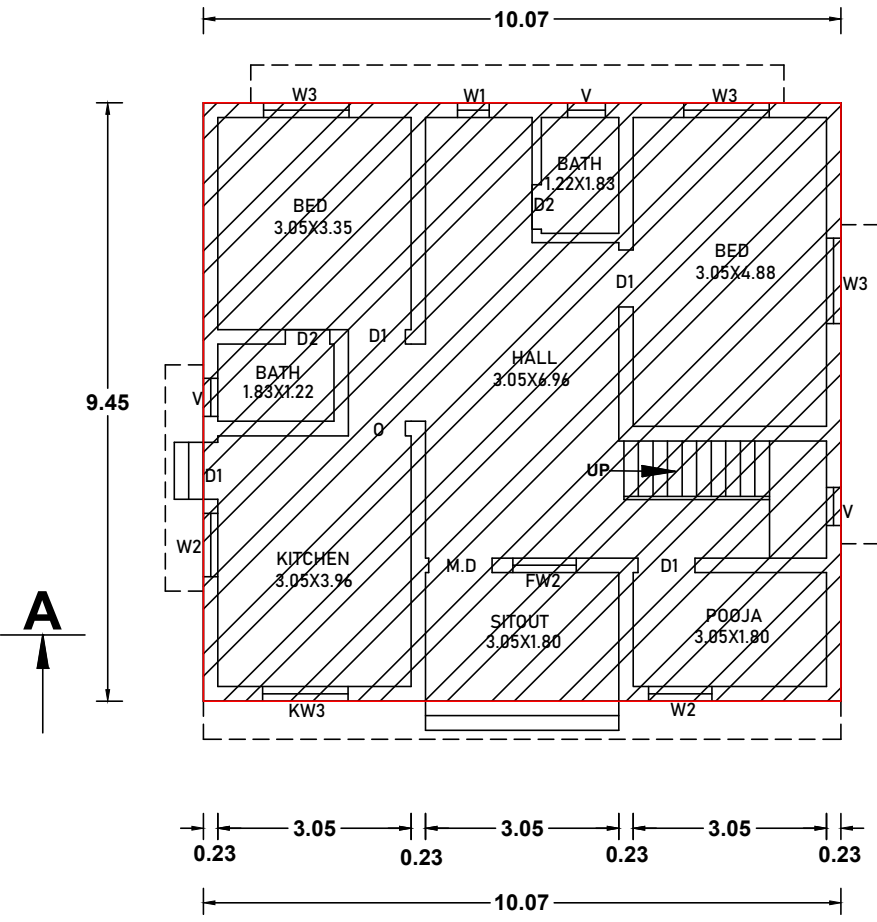
EXG.GROUND FLOOR PLAN
