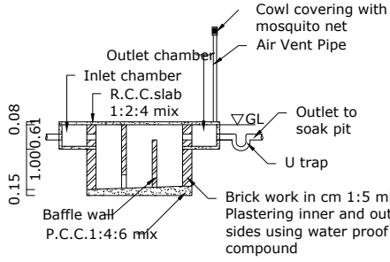
SECTION UV
