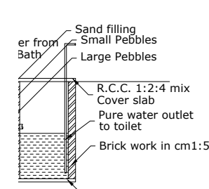
WATER RECYCLING SYSTEM
