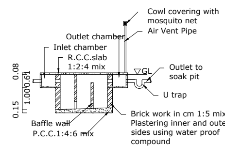
SECTION UV
