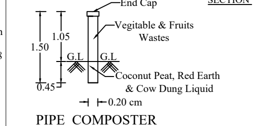
PIPE COMPOSTER
