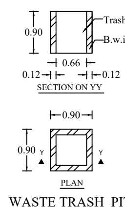
WASTE TRASH PIT
