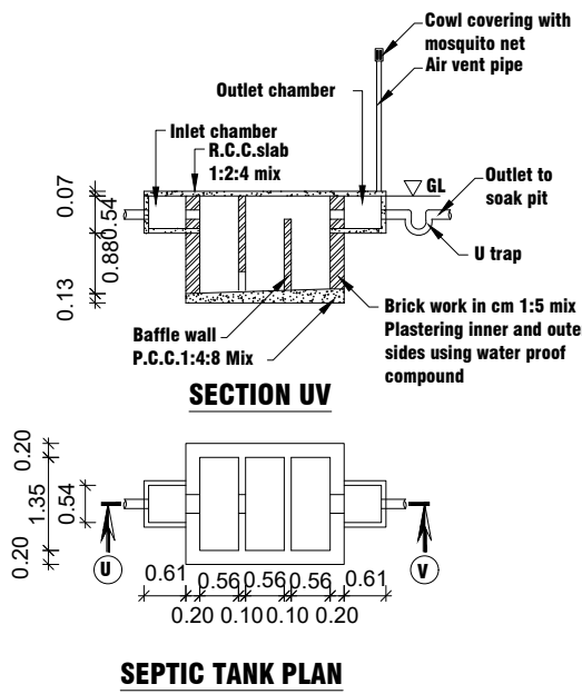
SECTION UV
