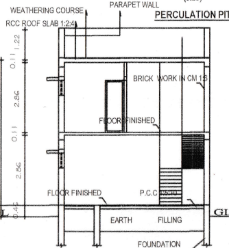
SECTION "A-B"
