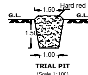
TRIAL PIT (Scale 1:100)
