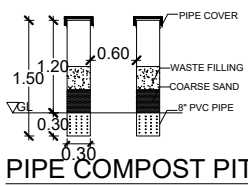
PIPE COMPOST PIT
