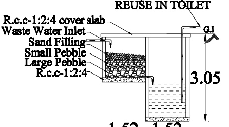
RECYCLING OF WASTE WATER KITCHEN & BATH ROOM
