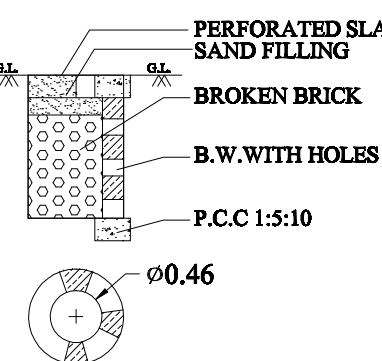
RAIN WATER PERCOLATION DRAWING TYPE -1A
