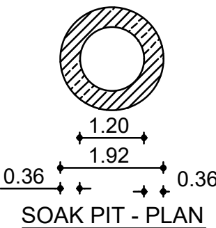
SOAK PIT - PLAN
