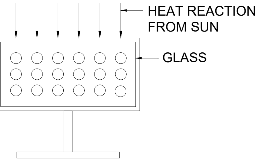
SOLAR SYSTEM
