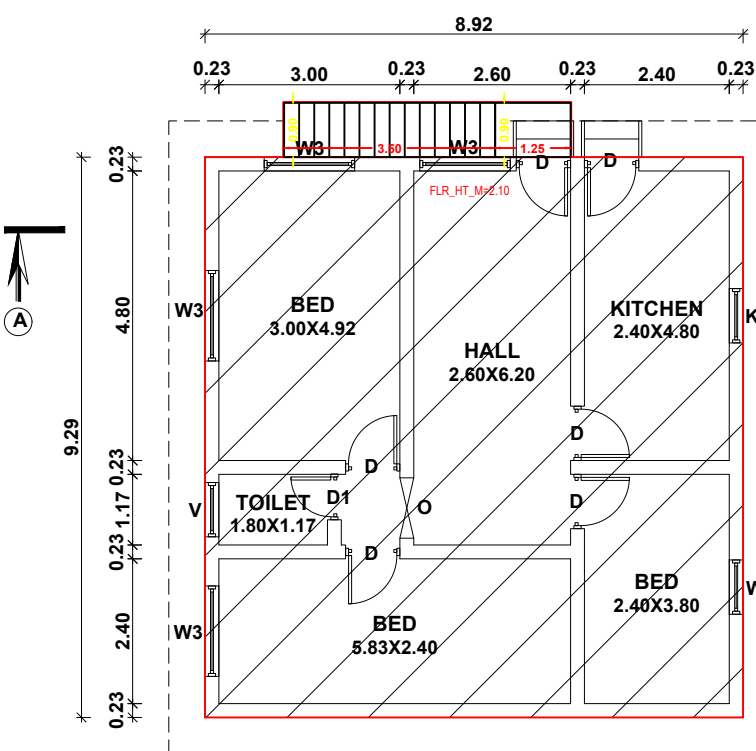
EX. GROUND FLOOR PLAN
