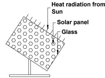
SOLAR SYSTEM
