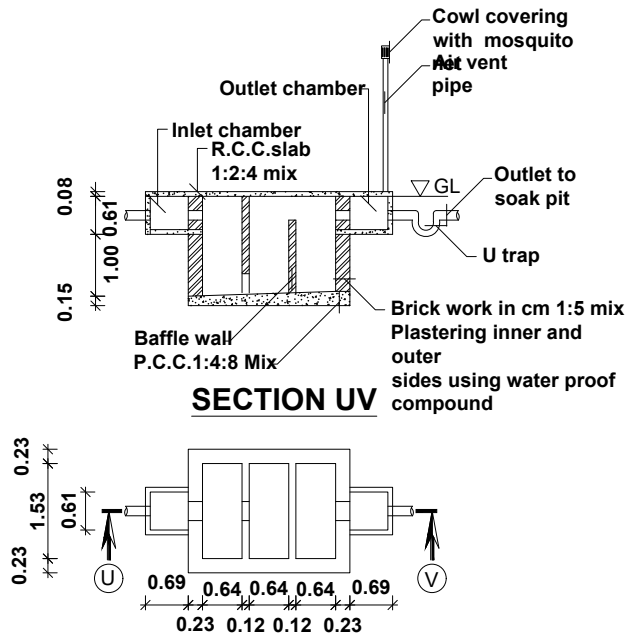
SECTION UV
