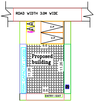
SITE PLAN
