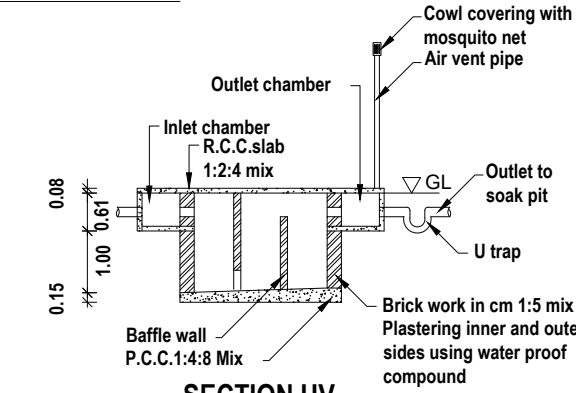
SECTION UV
