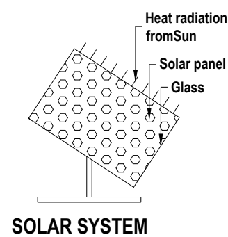
SOLAR SYSTEM
