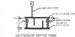
SECTION OF SEPTIC TANK
