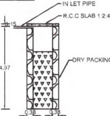
WASTE WATER TANK
