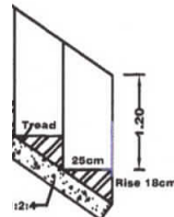
STAIR DETAILS
