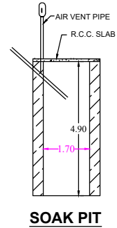
DETAILS OF RAIN WATER HARVESTING
