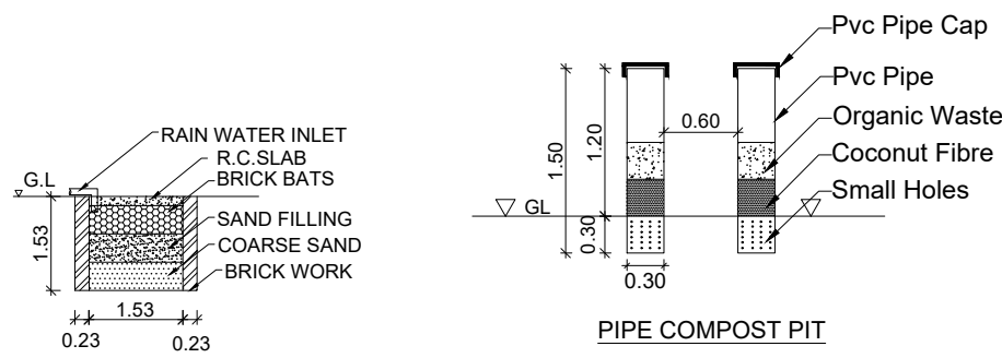
RAIN WATER STING PIT
