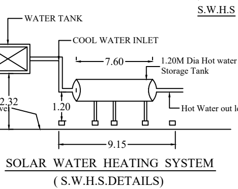
SOLAR WATER HEATING SYSTEM (S.W.H.S.DETAILS)
