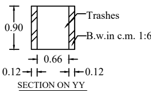
SECTION ON YY
