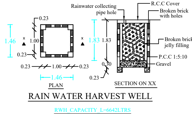
RWH CAPACITY: 1-6642LTRS
