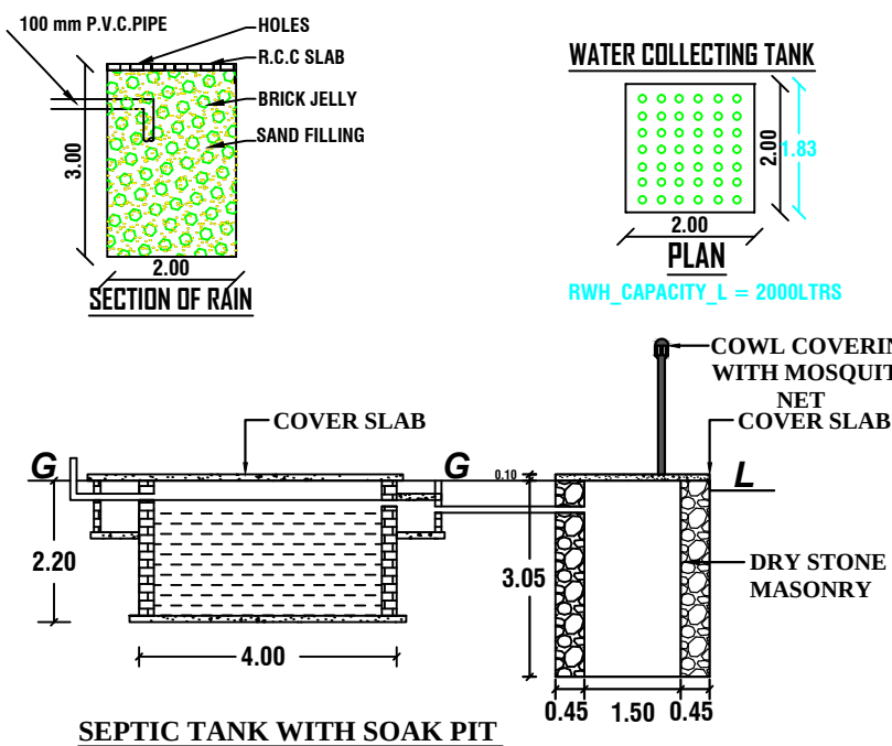
SEPTIC TANK WITH SOAK PIT
