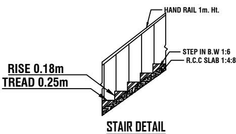
STAIR DETAIL
