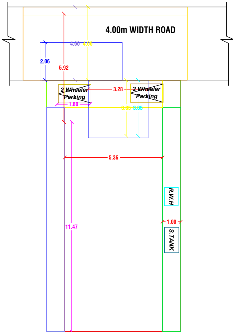
SITE PLAN
