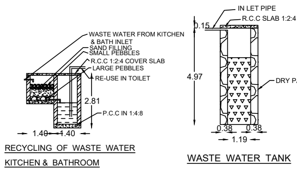
WASTE WATER TANK
