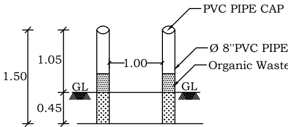
PIPE COMPOSED SYSTEM
