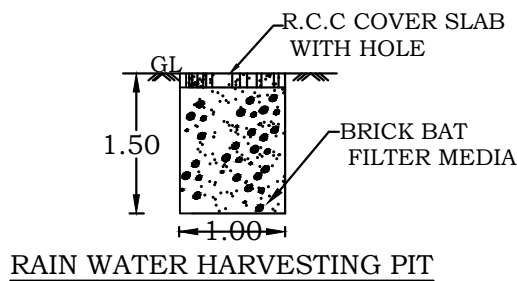
RAIN WATER HARVESTING PIT
