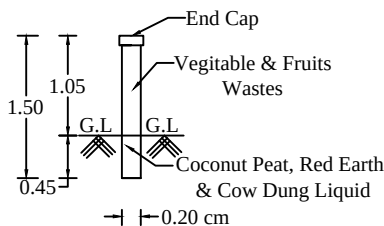
PIPE COMPOSTER
