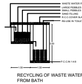
RECYCLING OF WASTE WATER FROM BATH
