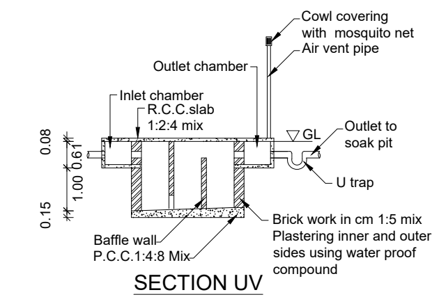
SECTION UV
