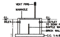
SECTION OF SEP.TANK
