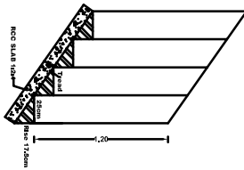
STAIR DETAILS
