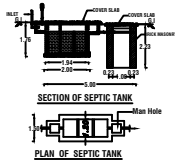
PLAN OF SEPTIC TANK
