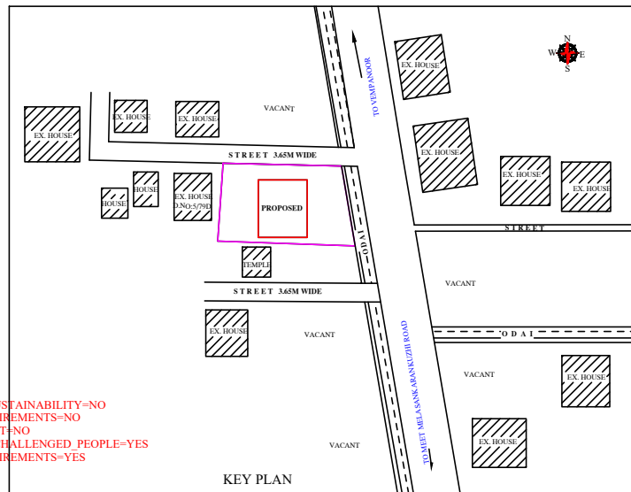
KEY PLAN
