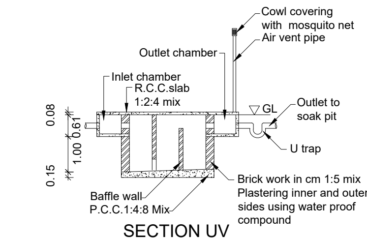
SECTION UV
