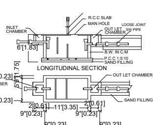
SEPTIC TANK:
