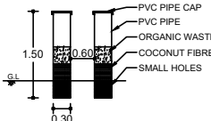
PIPE COMPOST PIT
