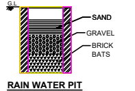
RAIN WATER PIT
