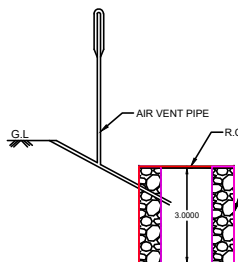
SECTION OF SOAKPIT
