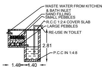
RECYCLING OF WASTE WATER
