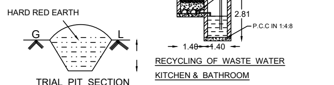
TRIAL PIT SECTION
