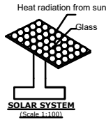
SOLAR SYSTEM (Scale 1:100)
