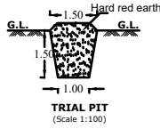
TRIAL PIT (Scale 1:100)
