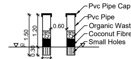
PIPE COMPOST PIT
