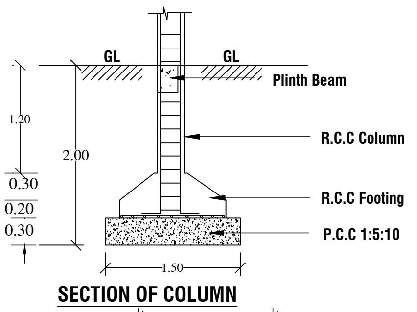
SECTION OF COLUMN
