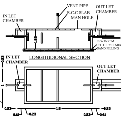
PLAN : SEPTIC TANK NOT TO SCALE
