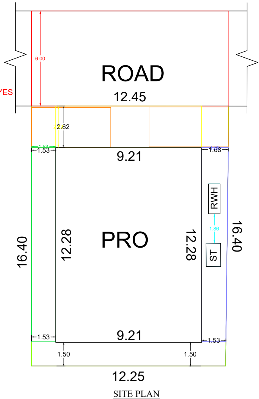
SITE PLAN
