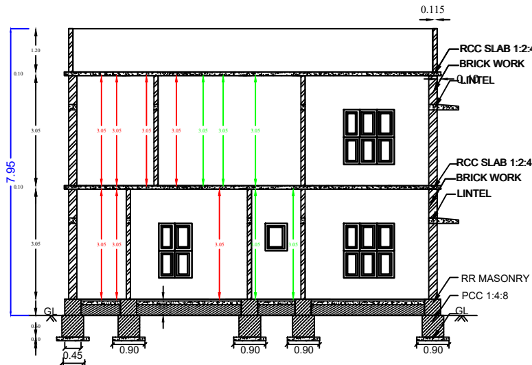
SECTION @ X-X'
