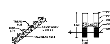
STAIRCASE DETAILS
