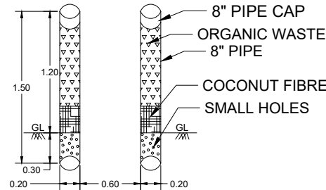
PIPE COMPOSITE PIT NOT TO SCALE
