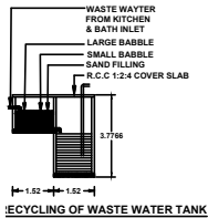
RECYCLING OF WASTE WATER TANK
