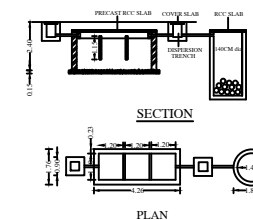
SEPTIC TANK
