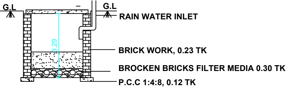
RAIN WATER HARVESTING RWH_CAPACITY_L=5000LTRS
