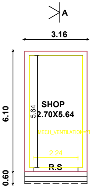
PLAN
