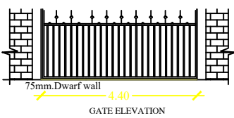
GATE ELEVATION
