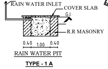
RAIN WATER PIT TYPE - 1A
