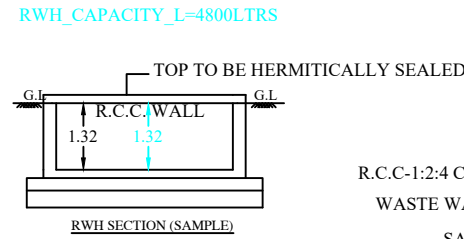
RWH SECTION (SAMPLE)
