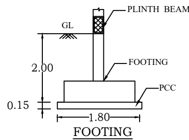
FOOTING
