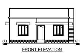
FRONT ELEVATION
