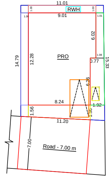
SITE PLAN
