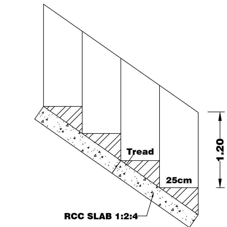
STAIR DETAILS
