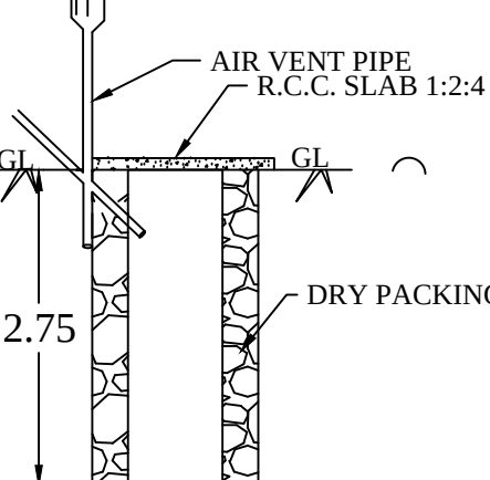
SOAK PIT DETAILS
