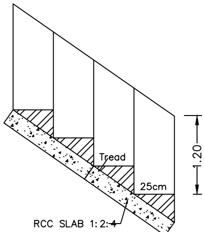
STAIR DETAILS
