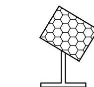
SOLAR SYSTEM ( Not to Scale )
