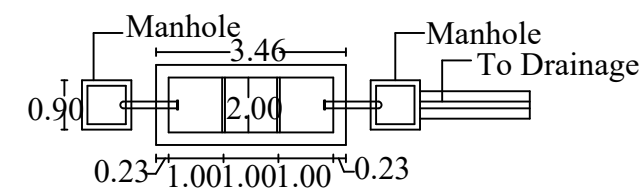
SECTION DETAILS OF SEPTIC TANK
