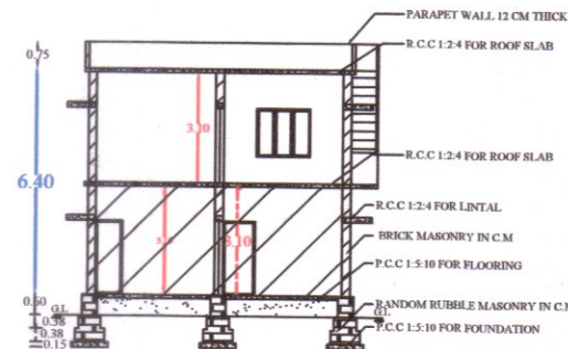
SECTION
