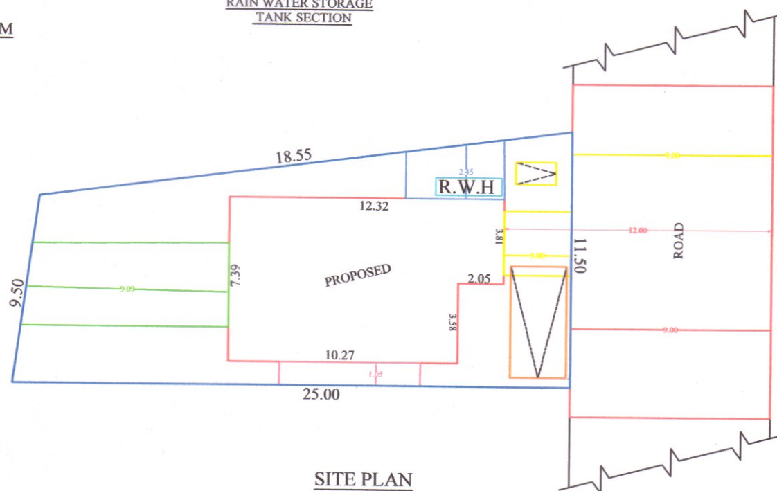
SITE PLAN
