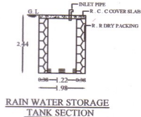
RAIN WATER STORAGE TANK SECTION
